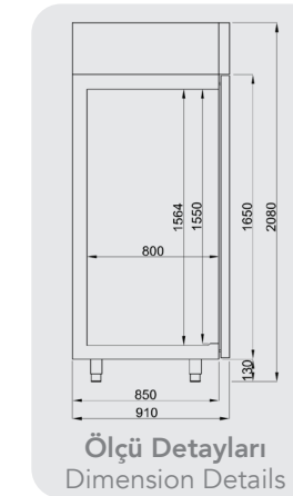
54 adet 36x17x12 Dondurma Kabi Kapasiteli 54 units 36x17x12 Ice Cream Cup Capacity
